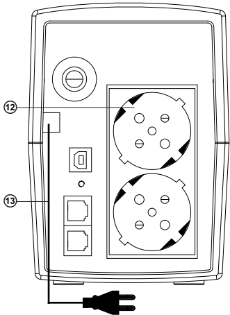
Pro 600/800/650 (LCD, USB) UPS Rear Panel
